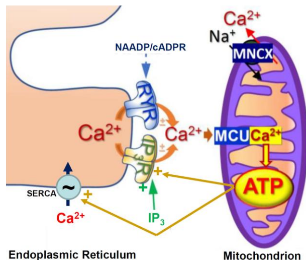
Fig. 1. Simplified diagram illustrating the close relationships between the signalling molecule \text{Ca}^{2+} and the primary energy carrier ATP. For details, see text. SERCA, \text{Ca}^{2+} ATPase in endoplasmic reticulum membrane; NAADP, nicotinic acid adenine dinucleotide phosphate; cADPR, cyclic ADP ribose; RyR, ryanodine receptor; \text{IP}_3 , inositol trisphosphate receptor; MNCX, mitochondrial \text{Na}^+/\text{Ca}^{2+} exchanger; MCU, mitochondrial \text{Ca}^{2+} uniporter.
